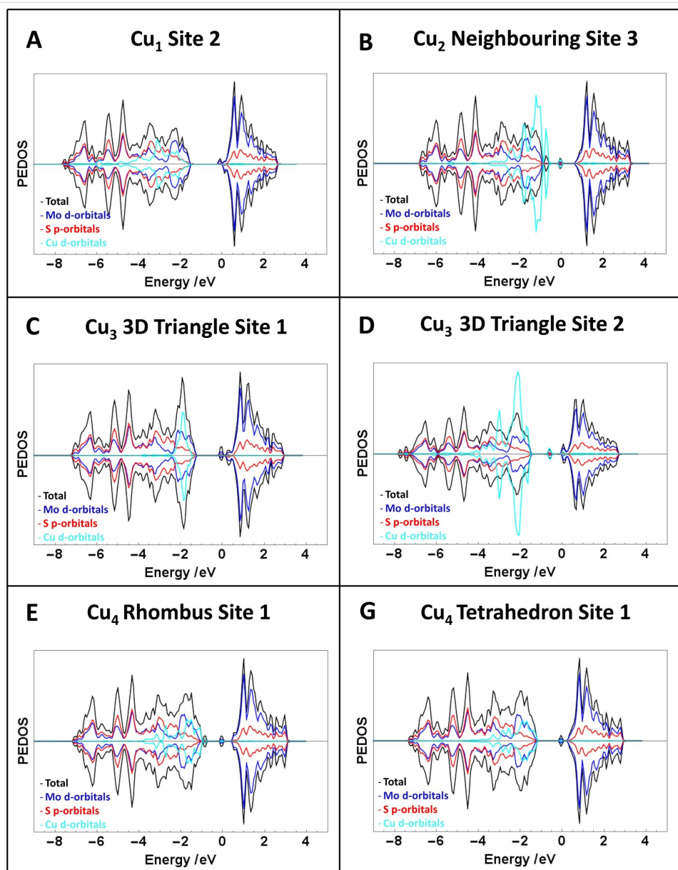
Figure 5: DOS plots of most favourable adsorption configuration for each Cu n structure on MoS 2 . The contribution of the Cu d orbitals has been increased by a factor of five for the ease of comparison and zero on the “energy” scale is the Fermi level.
