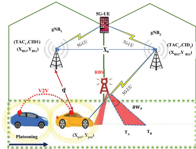
Fig. 5. RBS attack scenario, (X_{BS}, Y_{BS}) : location of the base station; T_A, T_B : edges of narrow beams; BW_\theta : beam width angles; V2V: Vehicle-to-Vehicle communications; TAC: Tracking Area Code; and, CID: Cell Identifier.
