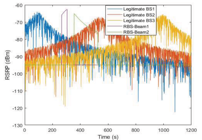
Fig. 6. Received signal strength for a mobile UE from a Rogue Base Station with two beams
