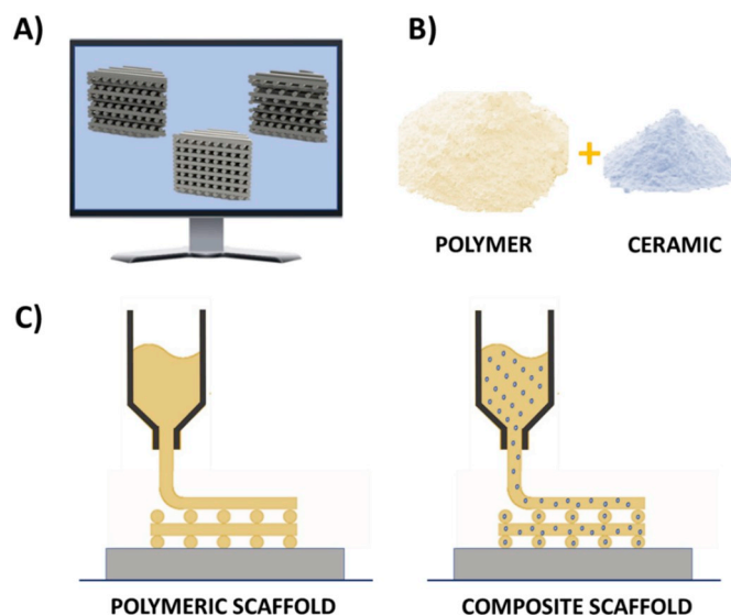
Fig. 1. 3D printed scaffold manufacturing route: A) scaffold CAD models, B) precursors' processing and C) extrusion-based scaffold 3D printing.
