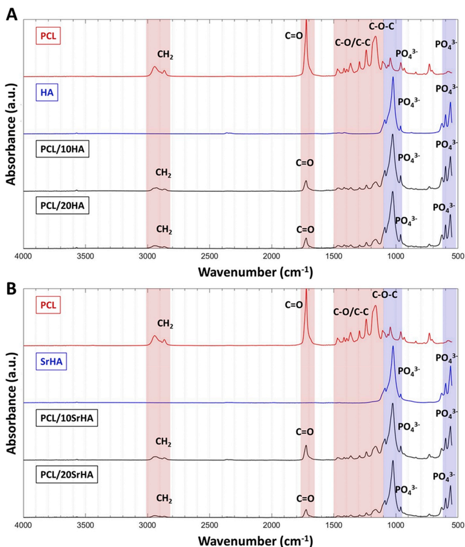
Fig. 4. FTIR spectra of A) PCL, HA and composite HA-based powders and B) PCL, SrHA and composite SrHA-based powders.
