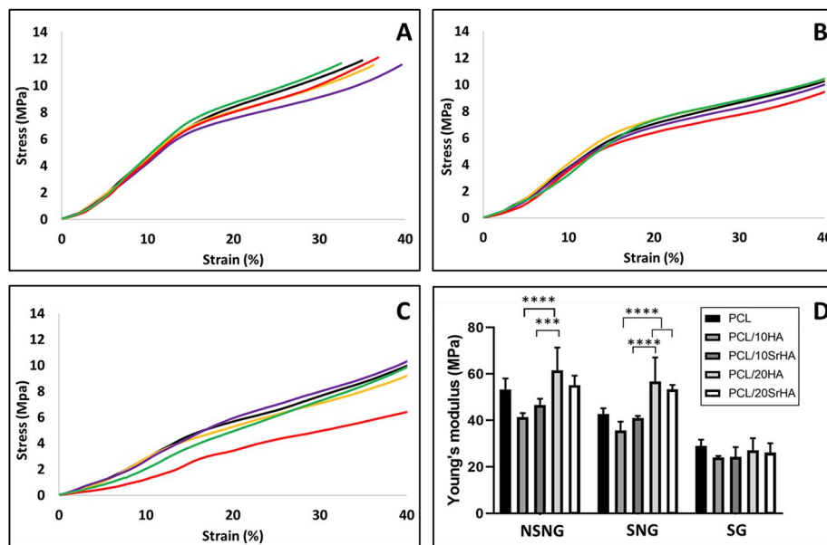
Fig. 6. Compressive stress-strain curves for: A) NSNG, B) SNG and C) SG architecture (— PCL, — PCL/10HA, — PCL/10SrHA, — PCL/20HA, — PCL/20SrHA) and D) Young's Modulus values of 3D printed scaffolds. Statistics: p < 0.0001 (****), p = 0.0005 (***).
