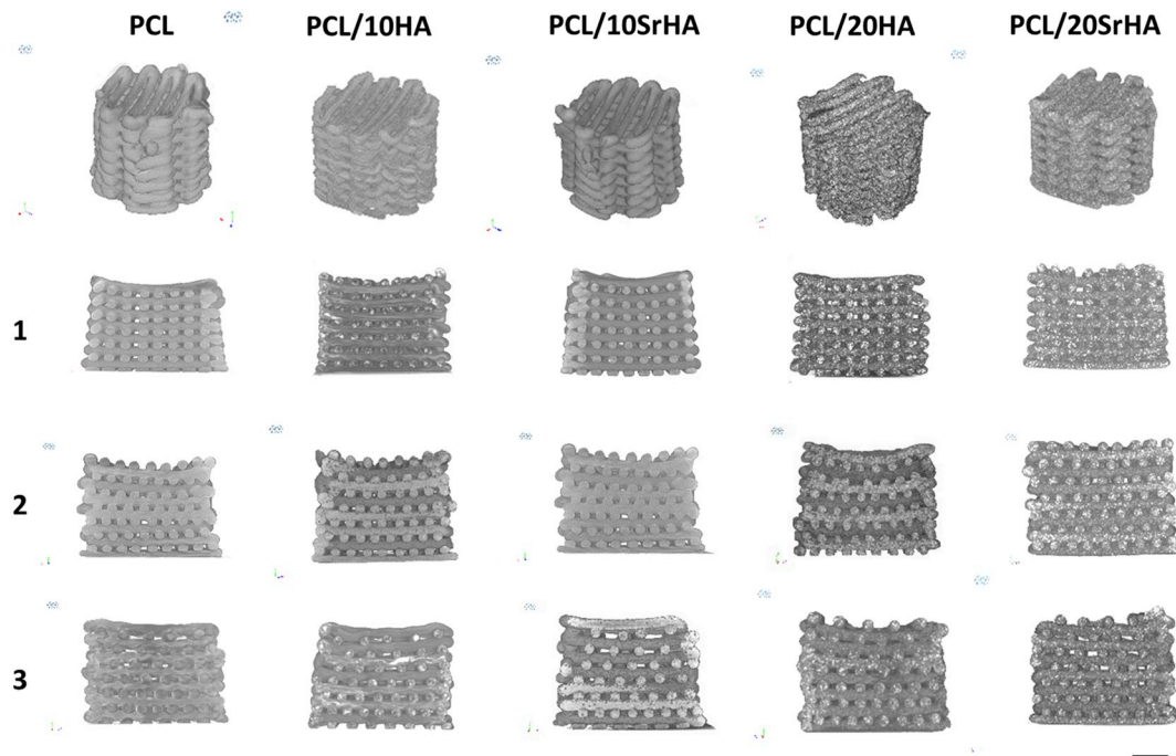
Fig. 5. Representative microCT images of all the 3D printed scaffolds and cross section of the three different architectures produced (1 = NSNG, 2 = SNG and 3 = SG architecture); [scale bar = 2 mm].
