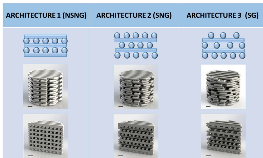
Fig. 2. 3D scaffold architectures (1 = NSNG, 2 = SNG and 3 = SG) and corresponding CAD model rendering of the 3D volume and cross section.
