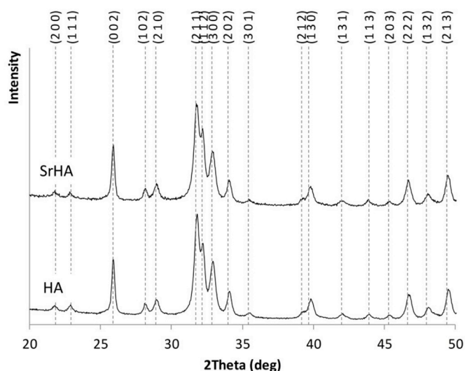
Fig. 3. XRD patterns of calcined (650 °C, 2 h) HA and SrHA powders.
