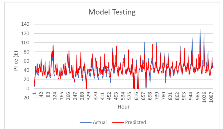
Fig. 1. Random Forest 24-Hour Model Testing
