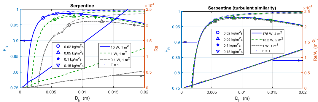
Figure 11. Heat recovery factor F_R for a square aspect ratio ( W=H ) serpentine tube absorber, R = 0.1 , with U_L = 3.8 \text{ W/m}^2\text{K} at various absolute pumping powers. Dotted lines show infinitely thick plate equivalent.
