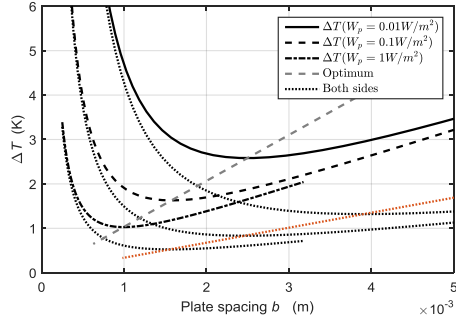
Figure 5. Comparison of \Delta T curves for a parallel plate collector when the fluid extracts heat from just one surface (bold) or both surfaces (dotted equivalents). (Fluid is Tyfocor-LS at 70°C, S^* = 750 \text{ W/m}^2 , L = 1 \text{ m} ).
