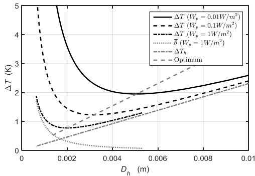
Figure 4. Difference in temperature \Delta T between fluid inlet and mean plate surface as a function of channel hydraulic diameter. This difference is the sum of a mean fluid temperature rise \Delta T_{fm} and the temperature difference necessary by virtue of the finite heat transfer coefficient, \Delta T_h . (Fluid is Tyfocor-LS at 70°C, S^* = 750 \text{ W/m}^2 , square microchannels, H = 1 \text{ m} , R = 0.637 ).
