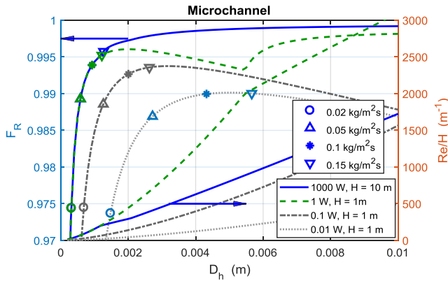
Figure 10. Heat recovery factor F_R as a function of hydraulic diameter with U_L = 3.8 \text{ W/m}^2\text{K} . for a 1 m wide microchannel plate with square passages; R = 0.637 , thickness \delta = 1.5b . The effects of transition commencing may be observed for the 1000 W and 1 W curves at D_h = 0.001 and 0.0053 \text{ m} respectively. Aluminium plate, k = 222 \text{ W/m}^2\text{K} ( F' = 0.994 at D_h = 0.005 \text{ m} ).
