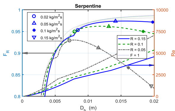
Figure 12. Effect of varying the diameter to pitch ratio R . ( W_{TOT} = 0.1 W, WH = 1 m 2 ).
