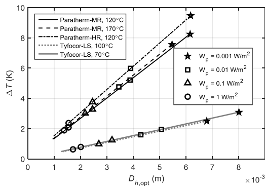
Figure 6. Optimum microchannel hydraulic diameter, at various pumping powers ( L = 1 m), for different liquids and temperatures. The higher viscosity fluid (Paratherm) requires a higher pumping power than Tyfocor to achieve the same \Delta T . [Square channels, constant R (any fixed value)].
