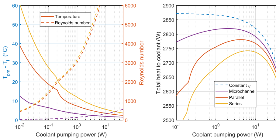
Figure 1. Effect of varying pumping power on \Delta T = T_{pm} - T_i and on overall heat flux to coolant. At low flow rates the increased plate mean temperature T_{pm} leads to increased heat loss and lower efficiency.
