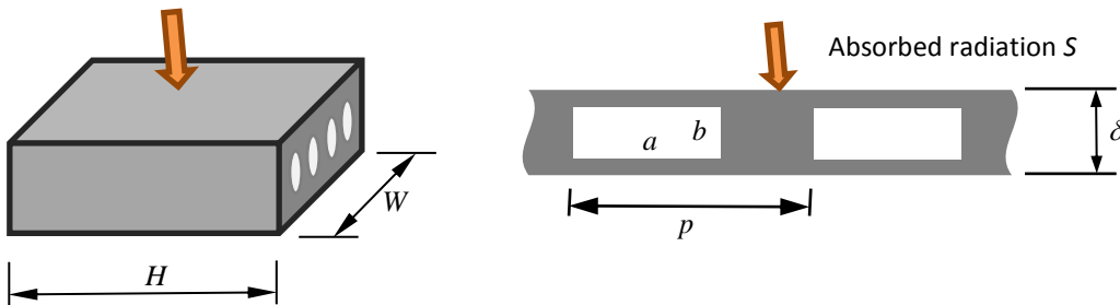
Figure 3. (a) Virtual plate with circular channels, (b) Nomenclature for a rectangular channel cross-section which may be modelled as an array of circular holes of equivalent area and perimeter. The passage side half-thickness t_s and top plate thickness t_t are defined as p = a + 2t_s , \delta = b + 2t_t .
