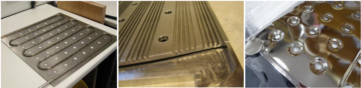
Figure 2. Examples of the three kinds of solar absorber. (a) Serpentine tube on plate, (b) Microchannel, prior to adding top cover, (c) Flooded panel. Experimental details and results will be reported elsewhere.
