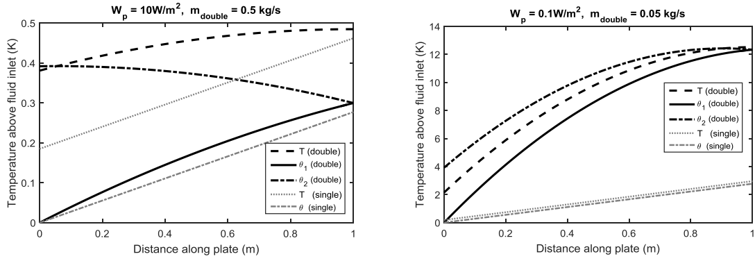
Figure 8. Metal ( T ) and fluid ( \theta ) temperature distributions along single and double-pass microchannel plates (a) high flow rate, (b) low flow rate. Square channels, R = 0.637 , D_h = 1.6 \text{ mm} , plate height = 1 m, Tyfocor-LS, S^* = 750 \text{ W/m}^2 , equivalent to one layer and two layers of the stacked design, Figure 7(b).
