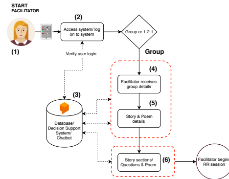
Fig. 1. Flow diagram depicting Digital Reading Room group session platform.
