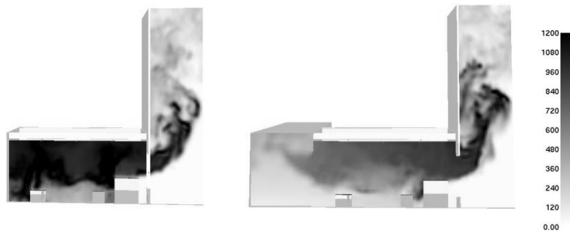
Figure 3: Predictions of gas mixture temperature ( ^{\circ}\text{C} ), 1000 s after fire initiation, for test case NoFD (left) and FD (right).
