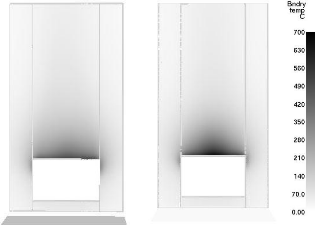
Figure 8: Predictions of facade wall temperature, 1000 s after fire initiation, for test cases NoFD (left) and FD (right).
