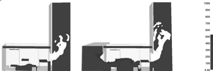
Figure 4: Predictions of EVF shape and location, 1000 s after fire initiation, for test case NoFD (left)
