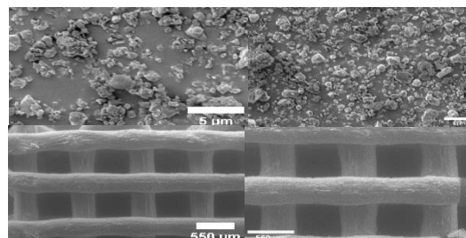
Figure 1 SEM imaging of TCP and Sr/TCP powders (top) and scaffolds produced (bottom).
