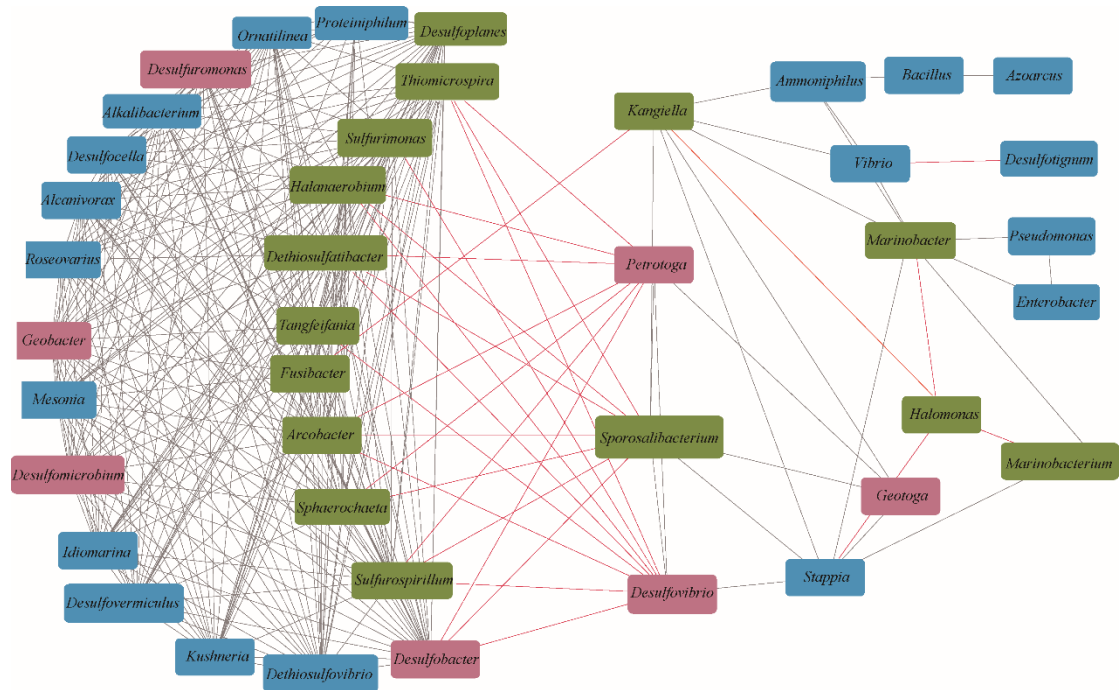
Fig. 5. The network inferences of dominant bacteria in the ESRB and ENRB enrichments and in the bioreactor. The nodes represent the dominant genus, and the connections between the nodes indicate a correlation between the two genera, the red line indicates a positive correlation, and the grey line indicates a negative correlation. The more connections through a node, the more associations the genus has with other members of microbial community.
