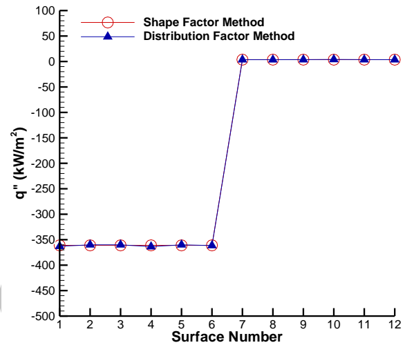
Fig. 3 Comparison of the heat fluxes obtained using the radiation distribution factor method and radiation shape factor method
