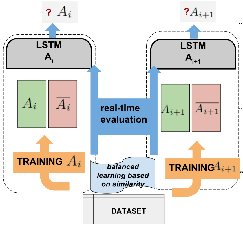
Figure 1. Scheme of ensemble of classifiers and balanced training for interleaved activity recognition. A_i and A_{i+1} represent different activities which can be activated in an interleaved way.
