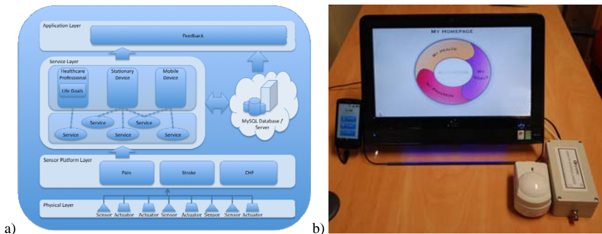
Figure 1: (a) Overview of the PSMS, comprising of the dataflow from sensor to server and server to database, (b) Second iteration of PSMS prototype containing smartphone, touchscreen and PIR sensor and receiver.
