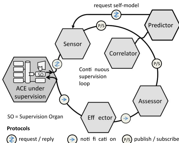
Figure 2 Organization of supervision components
