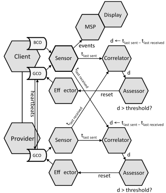
Figure 4 Dynamic Reconfiguration Scenario
