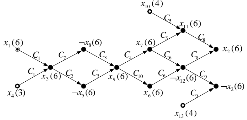
Implication Graph
