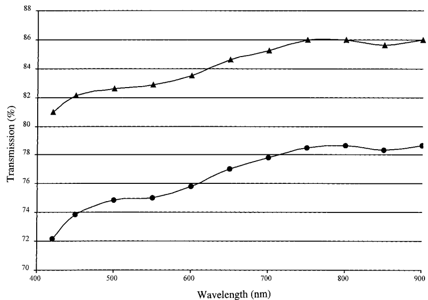
Fig. 4 Comparison of the transmission profiles between 400 and 900 nm for air- (●) and liquid-filled (▲) structures.
