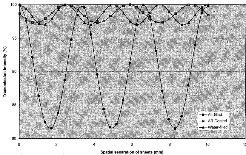
Fig. 2 Modelling the effect of spatial separation of the polycarbonate sheets as a function of transmission intensity.
