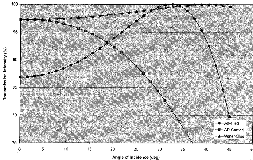
Fig. 3 Modelling transmission intensity as a function of incidence angle.
