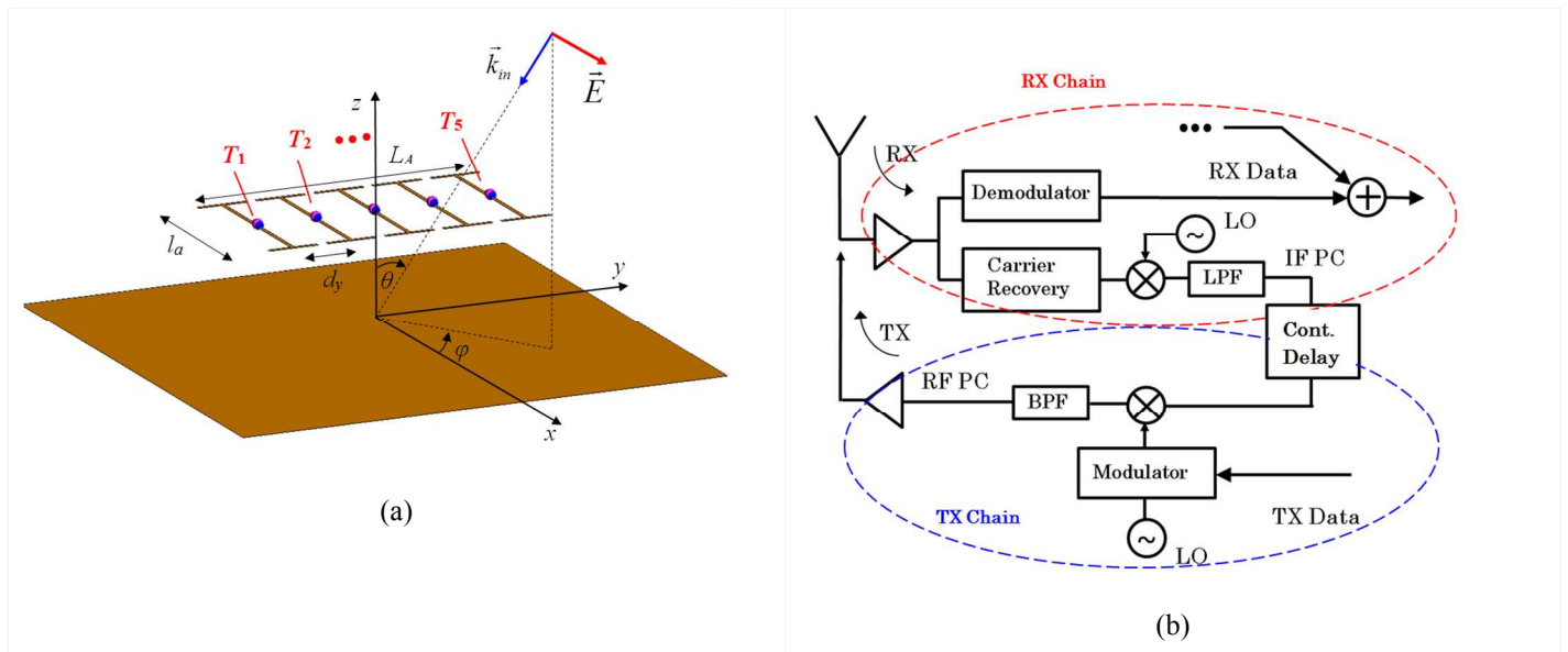
Fig.1. (a) A simulation model of an ultra-compact retrodirective antenna array illuminated by a linearly x -polarized monochromatic PW. The antenna array characteristic size L_a \sim N d_y \sim 0.5\lambda , N is a number of antenna elements, the inter-element spacings d_y are of order of 0.1\lambda . T_m , n=1,2,\dots,N are the PC antenna ports. The antennas are end-loaded to ensure electric
