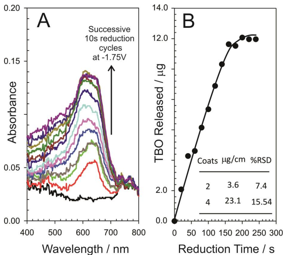
Figure 4. A) Spectra detailing the release of TBO after successive applications of a reducing potential (-1.75V for 10s increments) from a 5 cm length of 100 µm CAP coated gold wire. B) Yield of drug (µg) per 10s reduction cycle. Inset: Typical yield per length of suture depending on coating.
