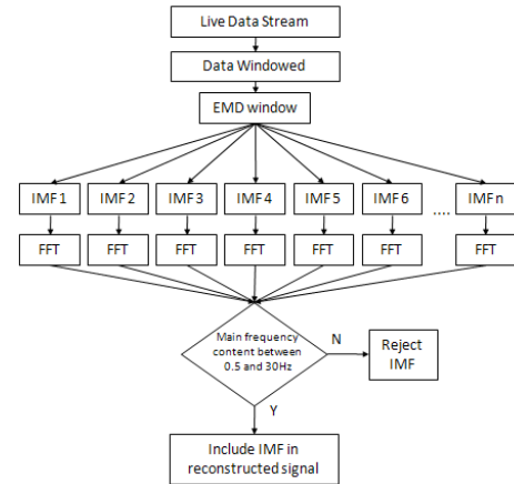
Figure 1. Dynamic EMD filter structure.
