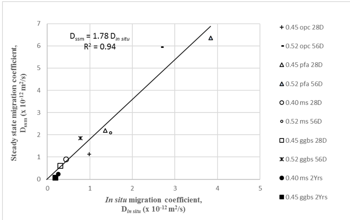
Fig. 5 – Graph demonstrating the usefulness of D_{in\ situ} in determining the steady state migration coefficient. (Legend shows, mix reference as in Table 2 + age of concrete at test, Example: 0.45 opc 28D – 0.45 w/b opc as in Table 2 tested at 28 days).
