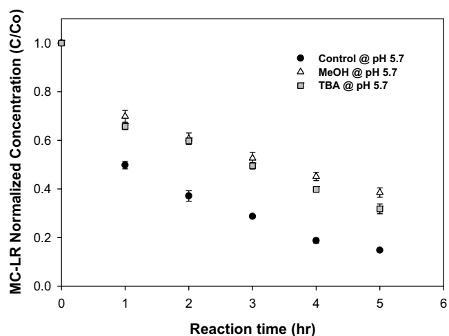
Fig. 1. Photocatalytic degradation of MC-LR with NF-TiO 2 in the absence and presence of methanol and tert -butyl alcohol as •OH scavengers under visible light at a) pH 3.0 b) pH 5.7.
