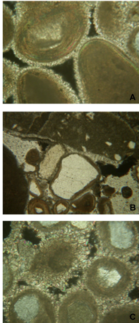
Fig. 4. Various cement types forming in the intertidal mixing zone. A – isopachous rim cement composed of microcrystalline HMC; B – small calcite crystals filling pore space in granular fabric; C – bladed aragonite crystals growing normal on surface of quartz grains.
