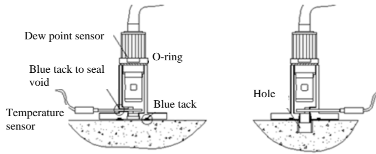
(a) Surface measurement (b) Measurement at different depths
