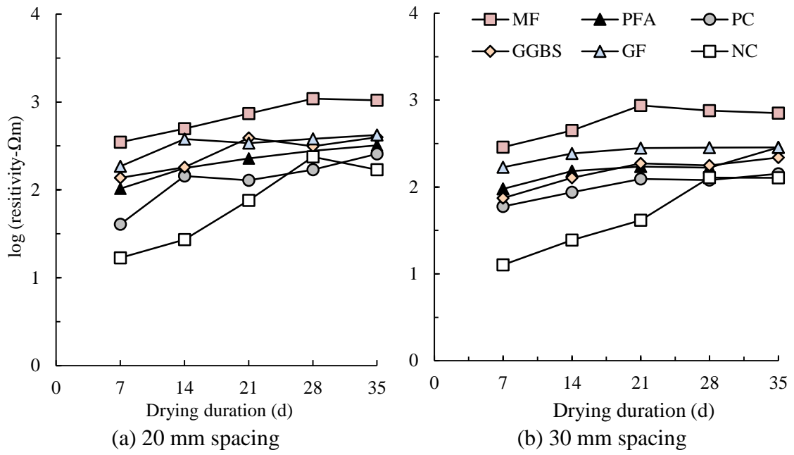
Figure 4 Influence of drying duration on surface resistivity
