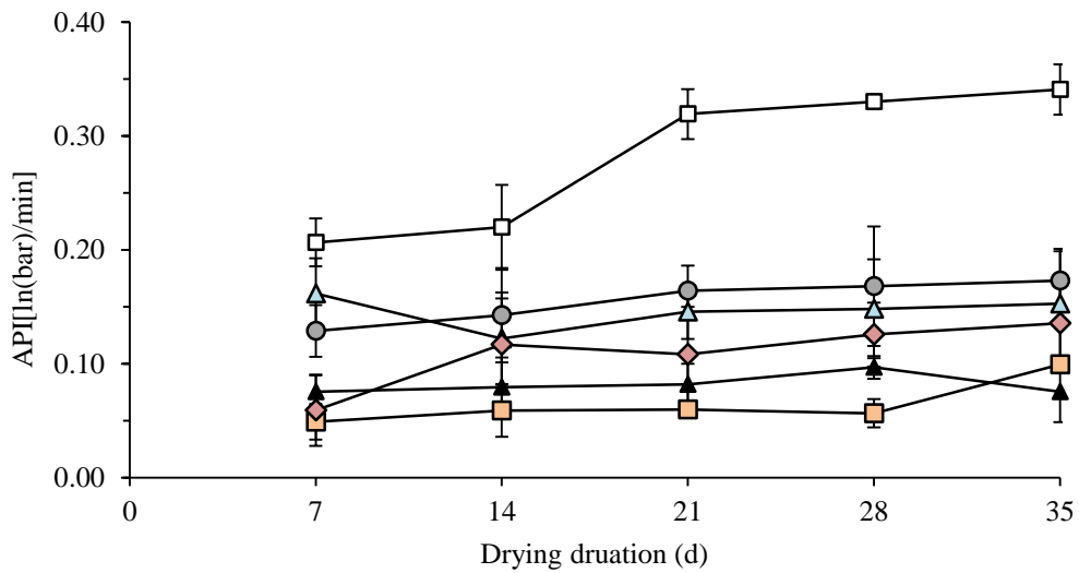
(c) Low volume test (LV)
