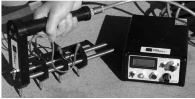
Figure 2 Surface resistivity meter
