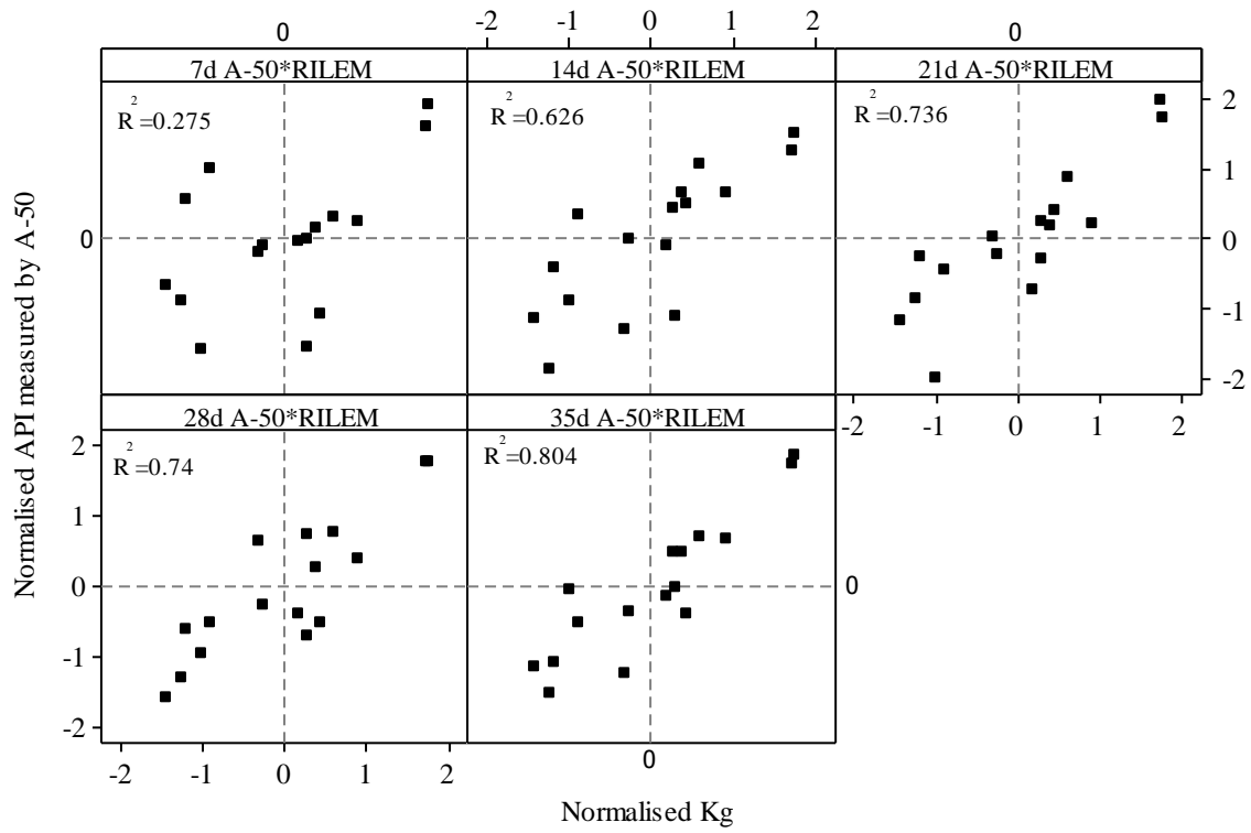
Figure 7 Effect of drying on relationship between A-50 and RIELM permeability tests
