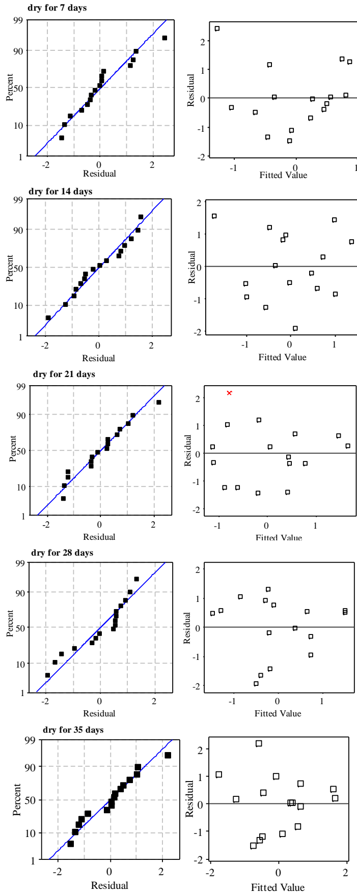
Figure 10 Diagnostic plots of regression analysis for LV test
