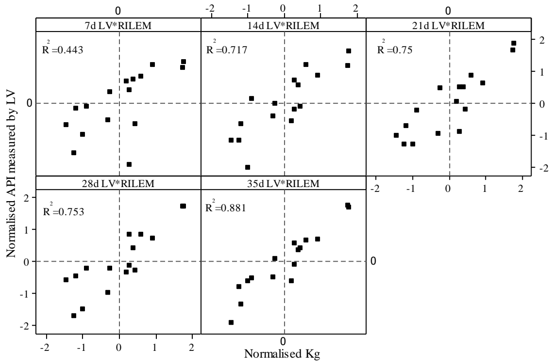
Figure 9 Effect of drying on relationship between LV and RILEM permeability tests
