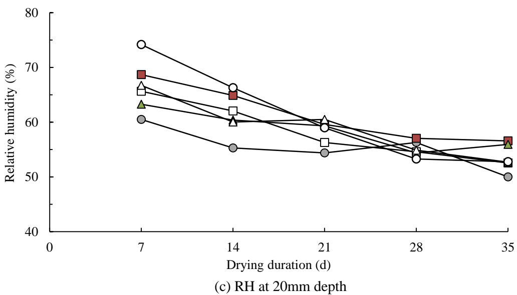
Figure 5 Relative humidity values at different depths after drying for different periods
