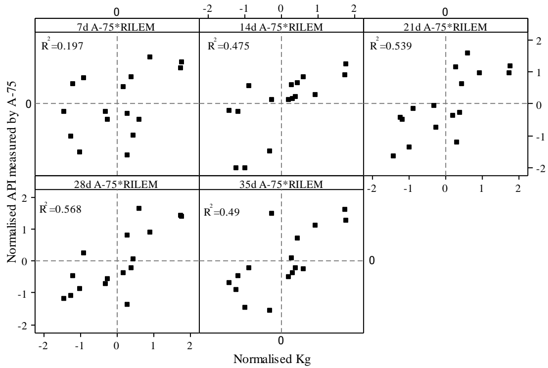
Figure 8 Effect of drying on relationship between A-75 and RILEM permeability tests
