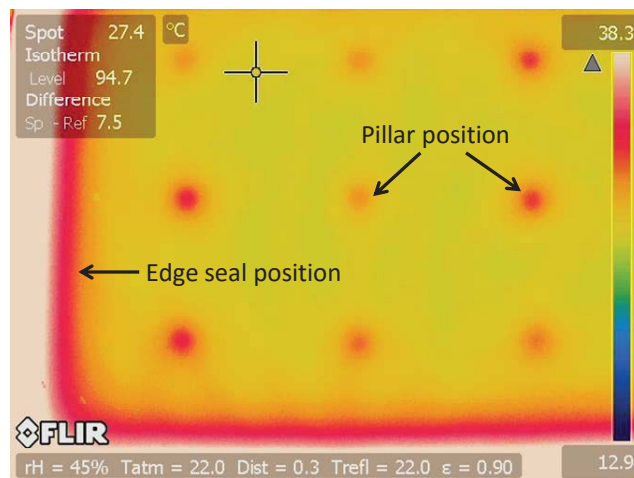
Fig. 7 IR-image of a flat vacuum panel
