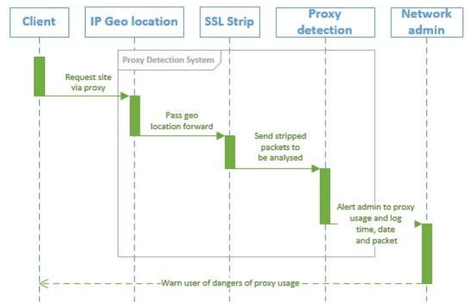
Fig 5: Sequence Interaction diagram
