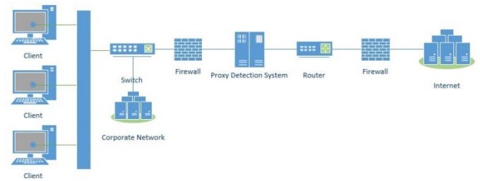
Fig 4: Network architecture
