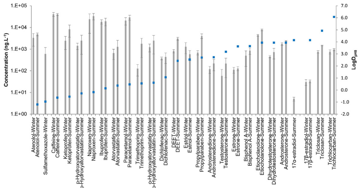
Fig. 1. Concentrations of TrOCs in the influent during different seasons ( 17\alpha -estradiol and sulfamethoxazole were not detected above its LOQ during the winter sampling).
