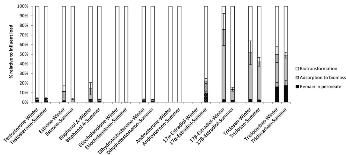
Fig. 3. Fate of hydrophobic TrOCs ( \log D_{pH8} > 3 ) through MBR treatment (pattern fill with dots denote values calculated from the LOQs when the concentrations in biomass and/or permeate were below the LOQs, so the percentage removal by the corresponding mechanism was below the values presented; 17 \alpha -estradiol was not detected above the LOQs in any influent samples during the winter sampling).
