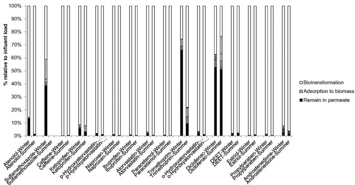
Fig. 2. Fate of hydrophilic TrOCs ( \log D_{pH8} < 3 ) through MBR treatment (pattern fill with dots denote values calculated from LOQs when the concentrations in biomass and/or permeate were below LOQs, so the percentage removal by the corresponding mechanism was below the values presented; Sulfamethoxazole was not detected above its LOQ in the summer sampling).
