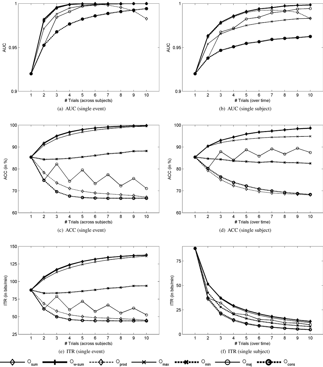
Fig. 1. SSVEP response detection results based on the AUC, the accuracy (ACC), and ITR. Figures 1(a) and 1(b): AUC for single-event detection as a function of the number of subjects and AUC for a single subject as a function of the number of trials, respectively. Figures 1(c) and 1(d): Accuracy for single-event detection as a function of the number of subjects and accuracy for a single subject as a function of the number of trials, respectively. Figures 1(e) and 1(f): theoretical ITR as a function of the number of subjects and the number of trials, respectively.
