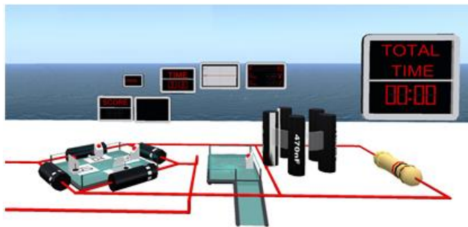
Figure 3 Graetz Bridge
