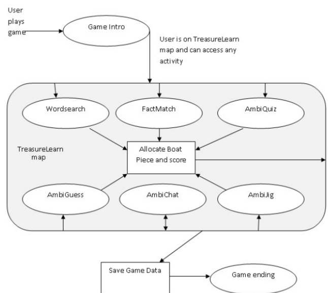
Figure 3 AmbiLearn ‘game play’ logic
