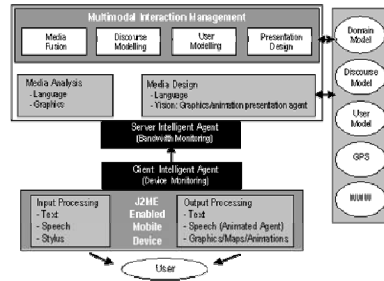
Figure 2. TeleMorph architecture.
