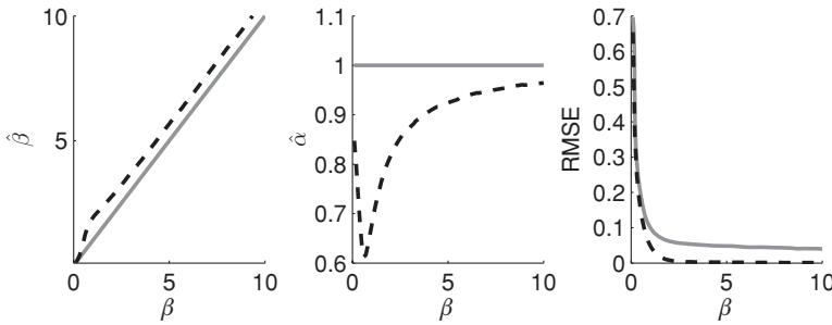
Fig. 4. SSE-minimizing parameters of the interrogation approximation to free response first-passage distributions are displayed for different signal-to-noise ratios ( \beta ) and fixed threshold-to-drift ratio \alpha . Left: Dashed line shows SSE-minimizing SNR \hat{\beta} ; true \beta is shown as solid line (of unit slope). Center: Dashed line shows SSE-minimizing threshold-to-drift ratio \hat{\alpha} ; true \alpha ( = 1 ) is shown as solid line. Right: Dashed line shows root mean squared error (RMSE) of the approximation using the SSE-minimizing parameters; solid line shows RMSE for the actual parameters.
