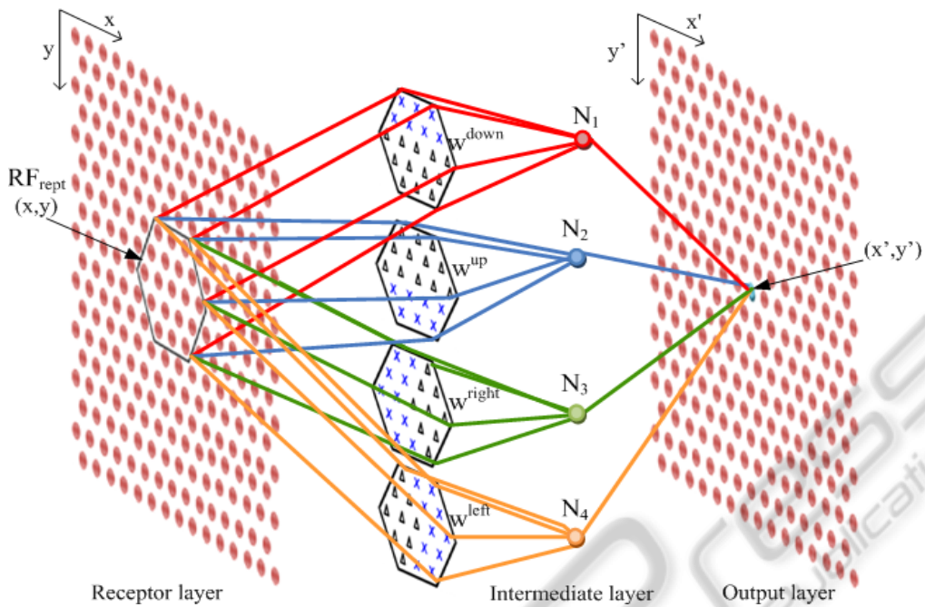
Figure 1: Spiking Neural Network Structure.
