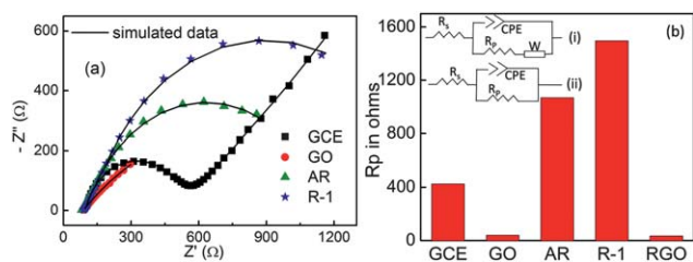
Fig. 4 (a) Nyquist plots of the impedance spectra obtained after each step in the fabrication process. The simulated data along with experimental points are shown in the same graph. GCE, GO, AR and R-1 represent bare GCE, GO modified GCE, AR antigen immobilized on GO/GCE and after addition of 25 \mu\text{g ml}^{-1} ( 0.17 \mu\text{M} ) of rabbit antibody solution, respectively. (b) Change in R_p at different stages of fabrication. The R_p obtained with the RGO modified GCE electrode is also shown for comparison with the GO modified electrode (the Nyquist plot for RGO/GCE is shown in Fig. 9). The inset shows the circuits used to model the sensor. Circuit (i) is used to model the AC response of the sensor with bare GCE, GO/GCE and RGO/GCE electrodes. Circuit (ii) is used after protein immobilizations.
