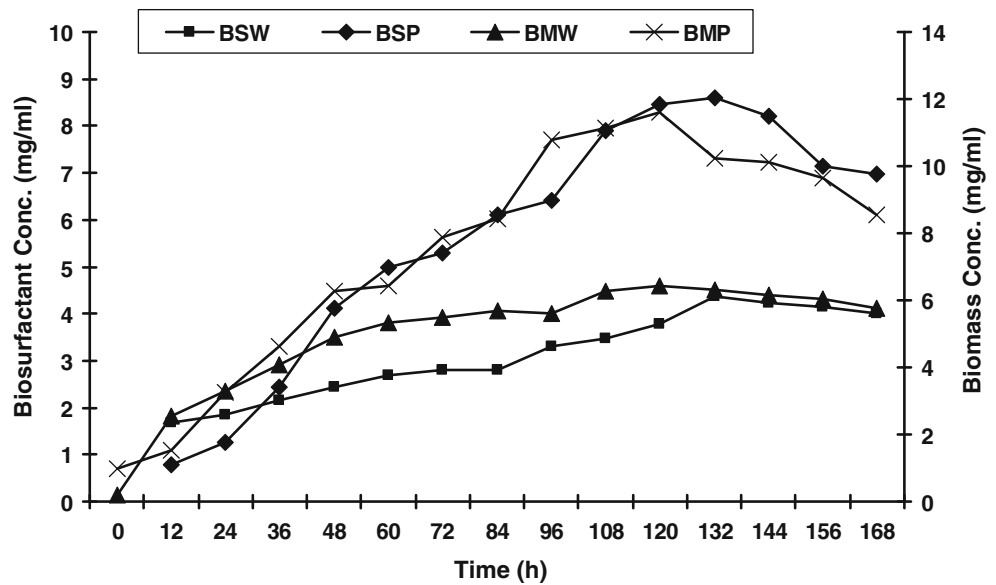
Fig. 1 Growth and biosurfactant production by P. aeruginosa in fermentor. BSW biosurfactant production using waste motor lubricant oil, BSP biosurfactant production using peanut oil cake, BMW biomass concentration with waste motor lubricant oil, BMP biomass concentration with peanut oil cake
