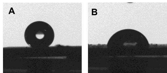
FIG. 4: (a) The static contact angle of the Untreated SWCNT and (b) the contact angle of the nitrogen plasma treated SWCNT.
