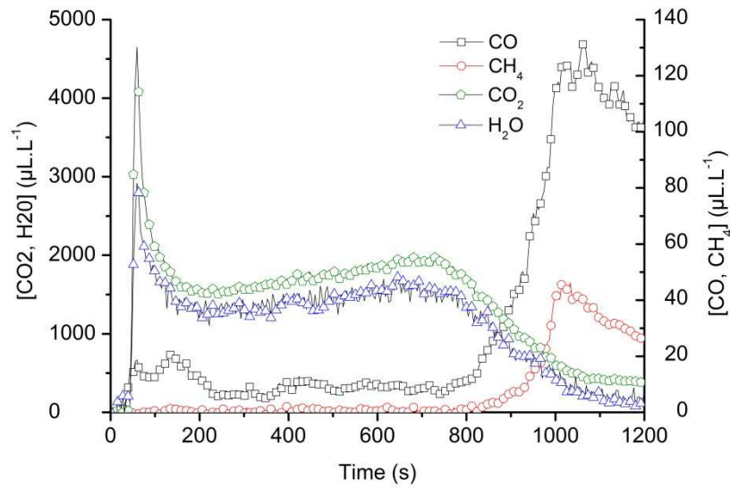
Figure 5: gaseous emissions and Mass Loss Rate during the thermal degradation of fir wood under cone calorimeter at 30\text{kW}\cdot\text{m}^{-2} .
