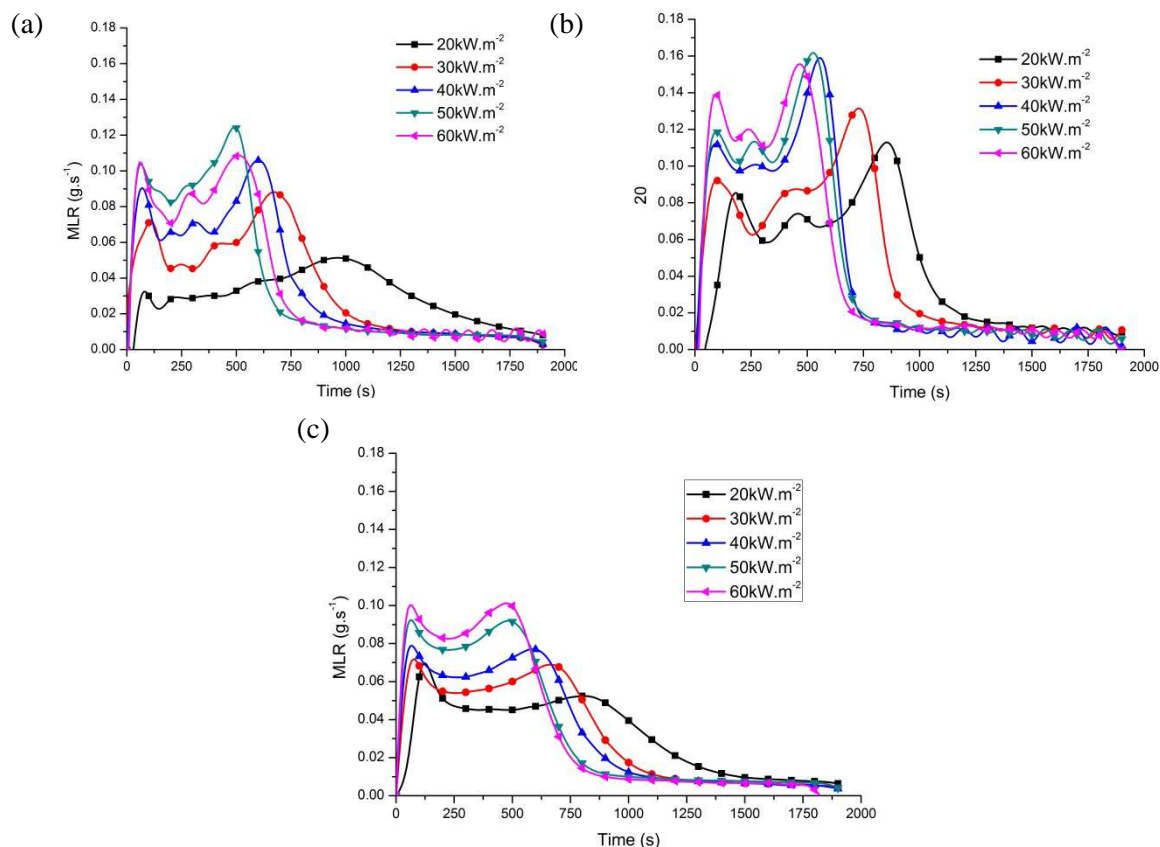
Figure 1: Mass Loss Rate evolution as function of time during the thermal degradation of different kind of wood (a: Plywood B, b: Plywood D, c: fir wood)
