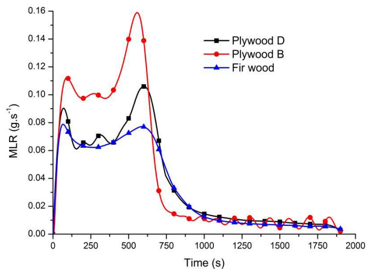
Figure 2: Comparison between curves at 30\text{kW}\cdot\text{m}^{-2}
