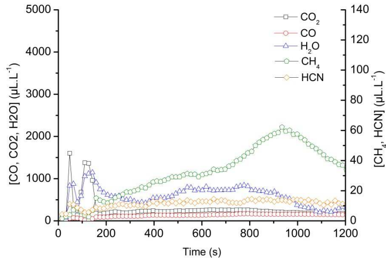
Figure 3: gaseous emissions and Mass Loss Rate during the thermal degradation of plywood B under cone calorimeter at 30\text{kW.m}^{-2} .
