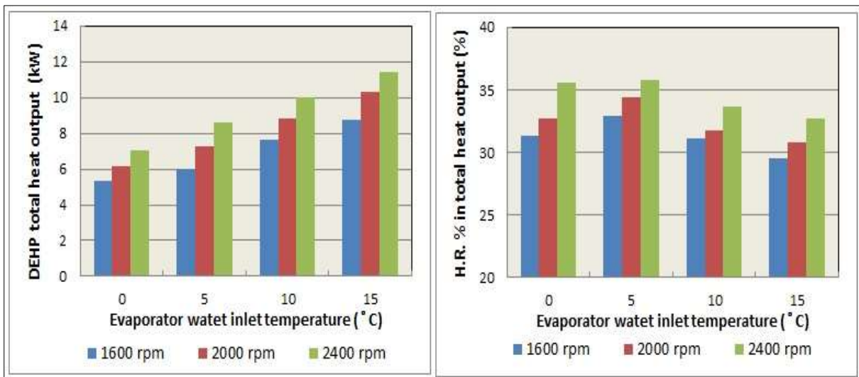
16 17 Figure 7 DEHP total heat output and heat recovery % in total heat output
