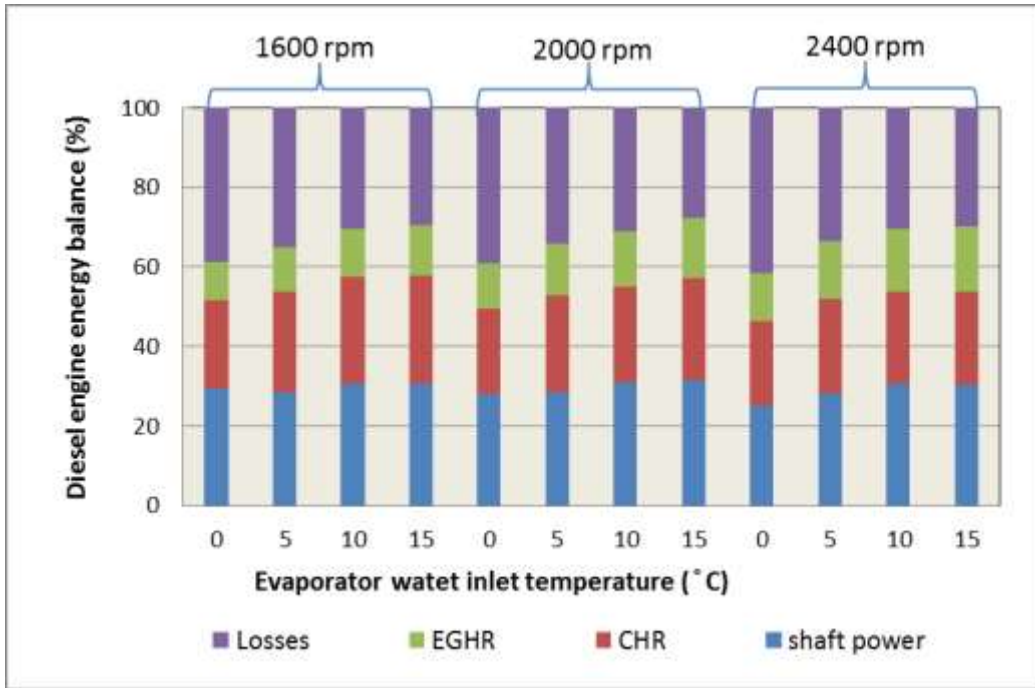
1 2 Figure 6 Diesel engine energy balance
