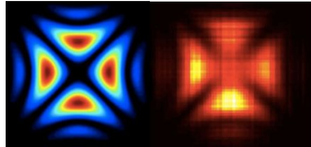
(a) (b) Fig. 12. (a) The theoretical predictions based on the Schrödinger equation and (b) the experimental imaging carried out by physicists at the University of Warsaw.
