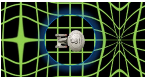
Fig. 17. The Alcubierre warp drive (Image source: https://www.universetoday.com/77005/astronomy-without-a-telescope-warp-drive-on-paper/ ).
